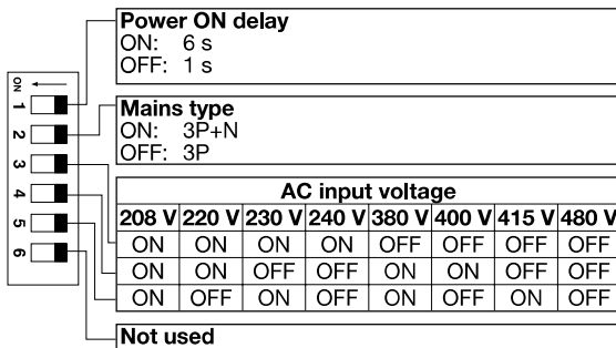
Fig. 3 DIP switch settings table M44
