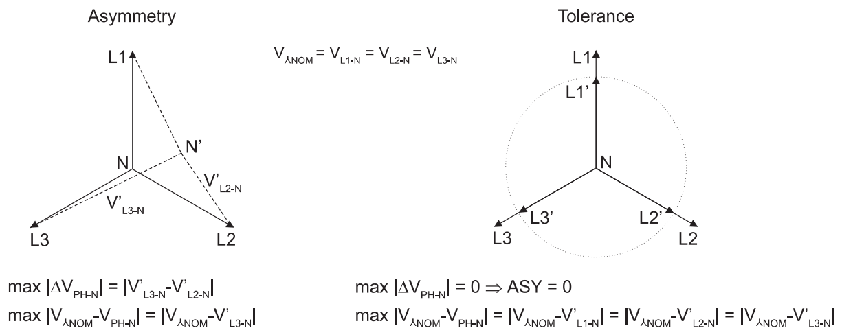
Fig. 2 Phase-neutral monitoring
