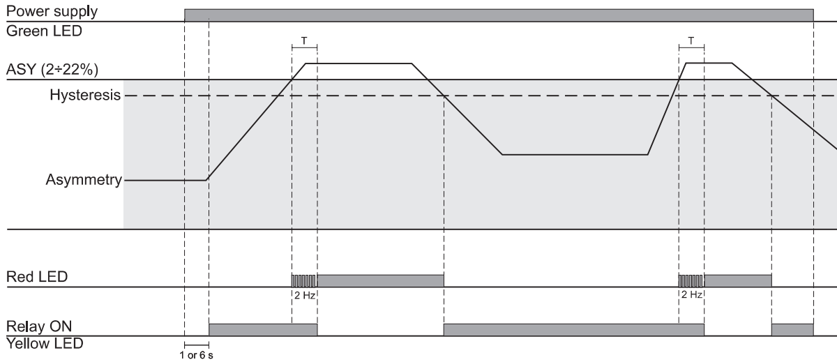
Fig. 6 Asymmetry monitoring
