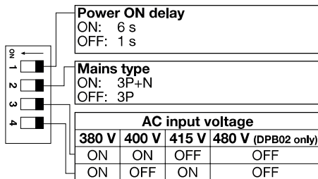
Fig. 5 DIP switch settings table M48
