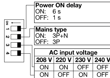
Fig. 4 DIP switch settings table M23
